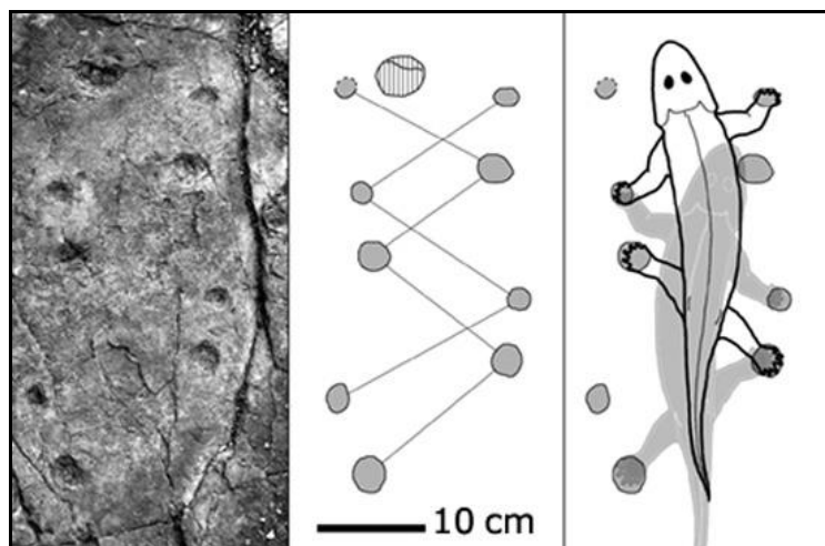
Fig. 6. The oldest tetrapods tracks present on dolomites bed-surface in Zachęlmie quarry (source: Niedźwiedzki at al. 2010)
