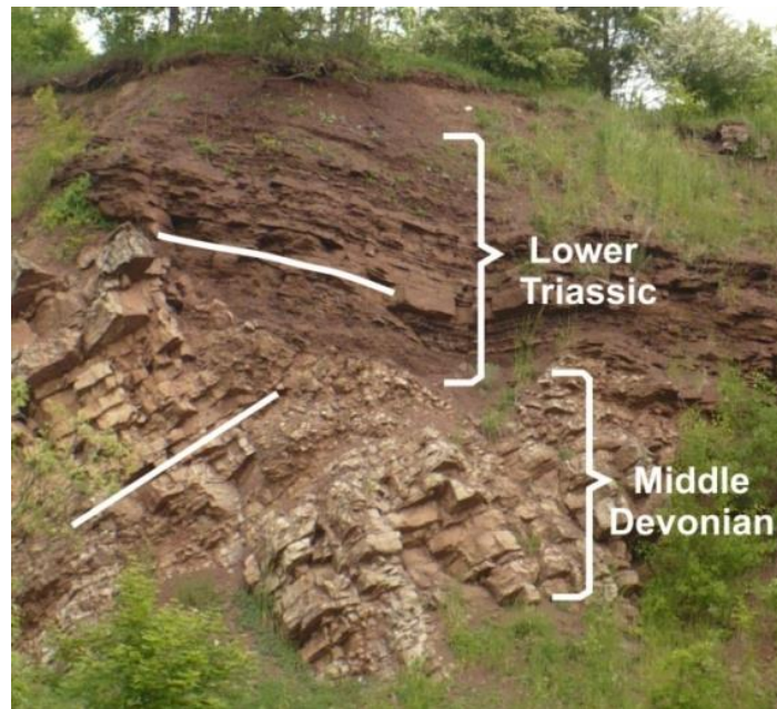
Fig. 5. Angular unconformity and stratigraphic gap exposed in Zachęlmie quarry (own elaboration)
