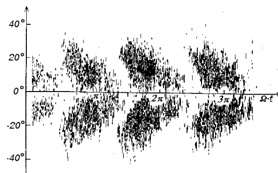
Fig. 1. Diagram of the "Maunder butterflies" [46], according to observations from 1874 to 1913, this shows the areas of existence of sunspots depending on the heliographic latitude (in the "royal zone") and phase of the solar cycle, \Omega t
