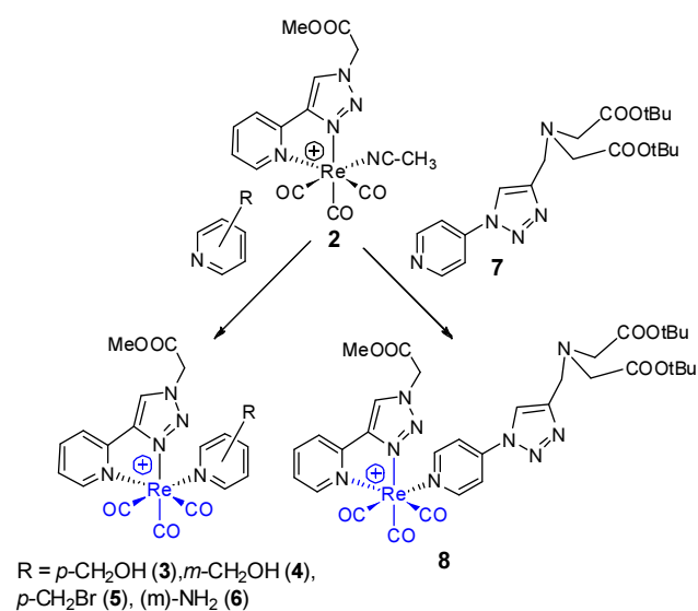
Figure 1. Synthetic pathways
