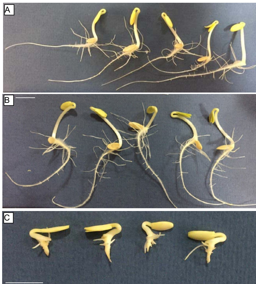
Fig. 2. Cucumis sativus sproutings (control) (A); with the addition of Pholiota squarrosa 2010 biomass (B) and Pholiota subochracea 2535 biomass (C); 3 days of germination, stroke length 1 cm
