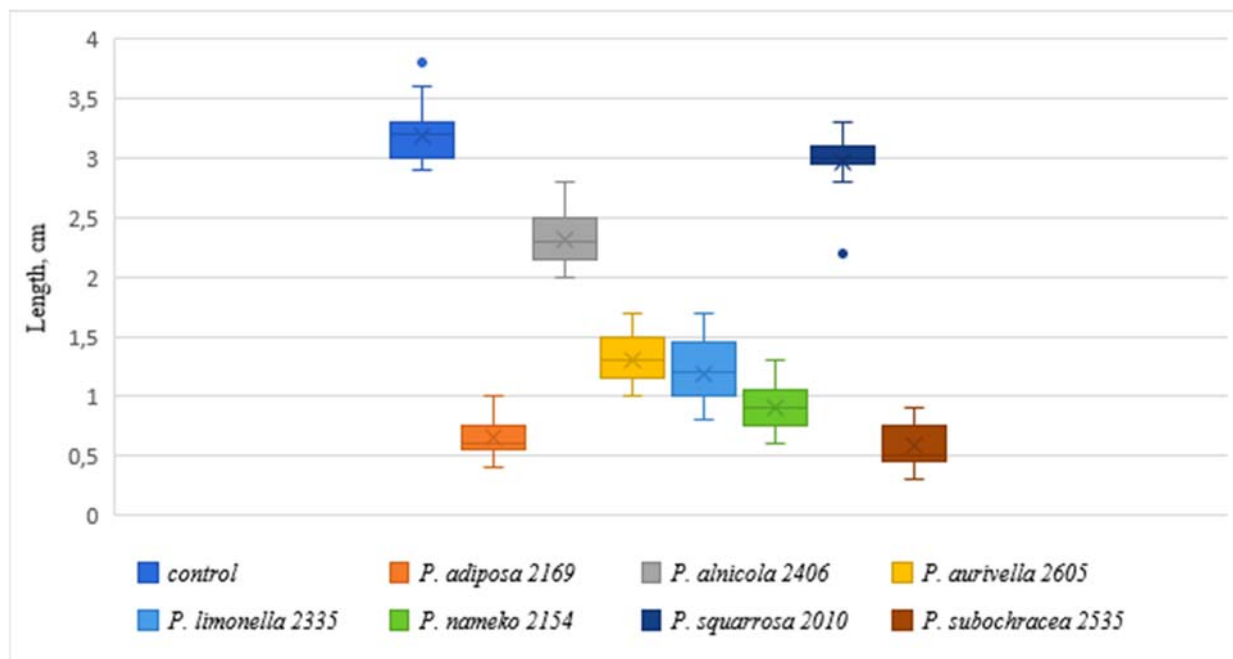
Fig. 4. Influence of Pholiota species biomass on the length of C. sativus shoots
