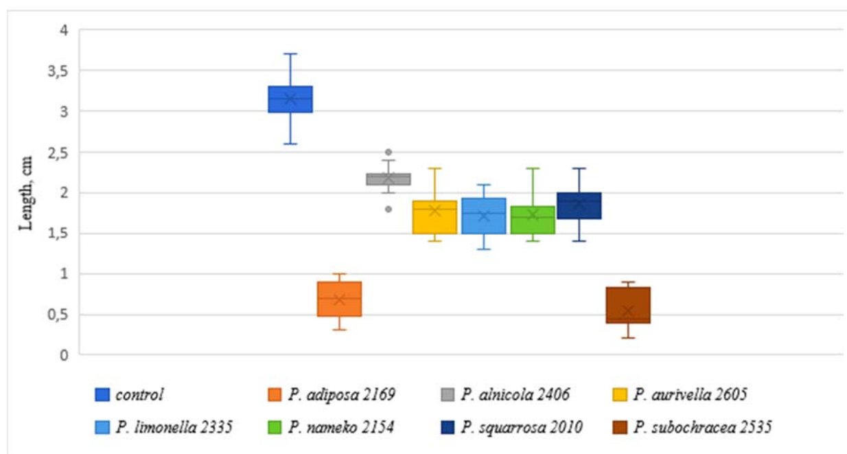
Fig. 8. Influence of Pholiota species biomass on the length of L. sativum shoots
