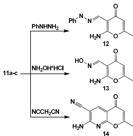
Scheme 4. Confirmation of aldehyde nature of derivatives 11a–c.
