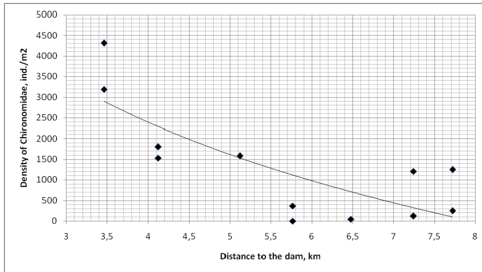
Fig. 2. The relationship between Chironomidae larvae density and distance from hydroelectric dam.
